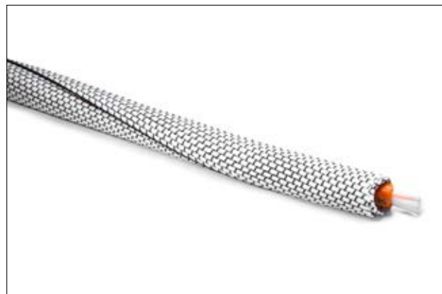
Rodent repellent self-closing sleeving in application with fibre optic cable.
